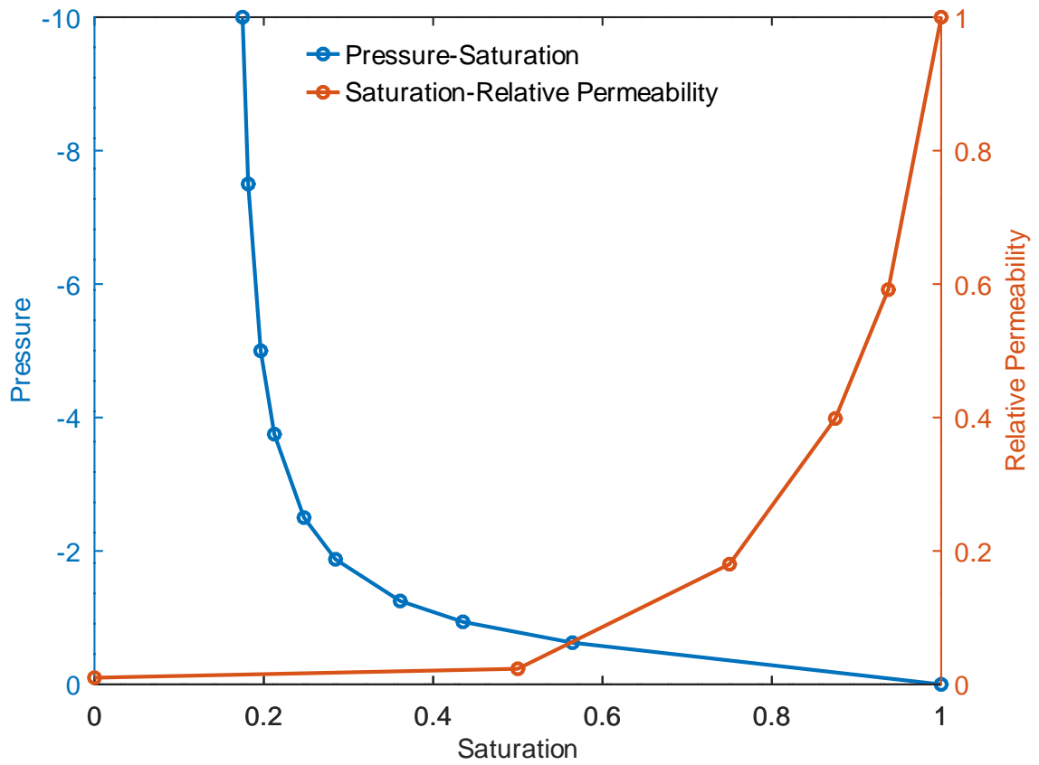
Figure 2.19: Example of using functional parameters to generate tabular constitutive relationships.
