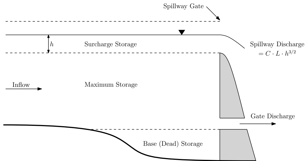
Figure 2.11: Diagram of a reservoir with a spillway.
