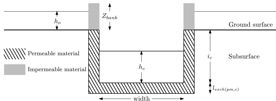
Figure 2.18: Rectangular 1-D channel cross section showing the stream bank height Z_{bank} , incision depth i_c , streambed thickness l_{exch(pm,c)} , overland head h_o , and channel head h_c .
