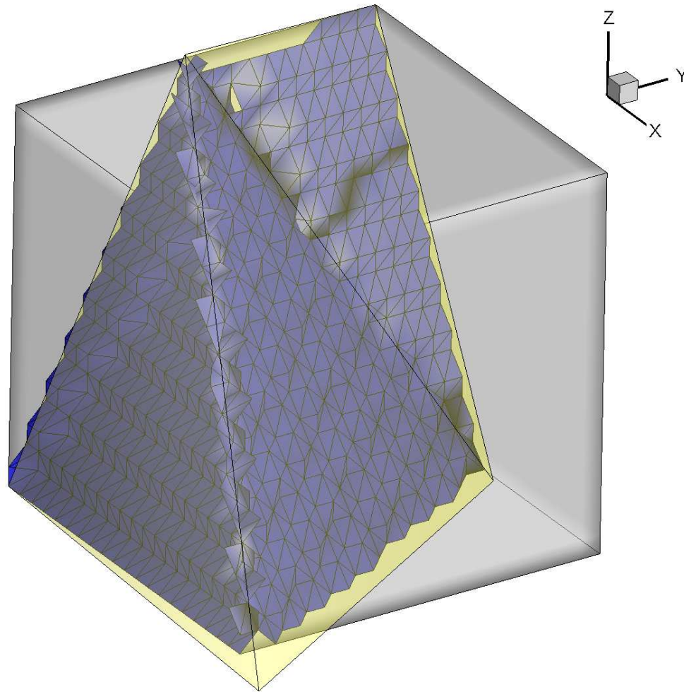
Figure 2.14: Example of fracture generation showing 3-D porous medium domain (grey cube), Tecplot triangles (yellow triangles), and the resulting fracture elements (blue triangles).
